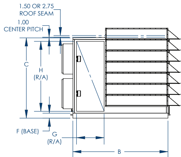
END VIEW
