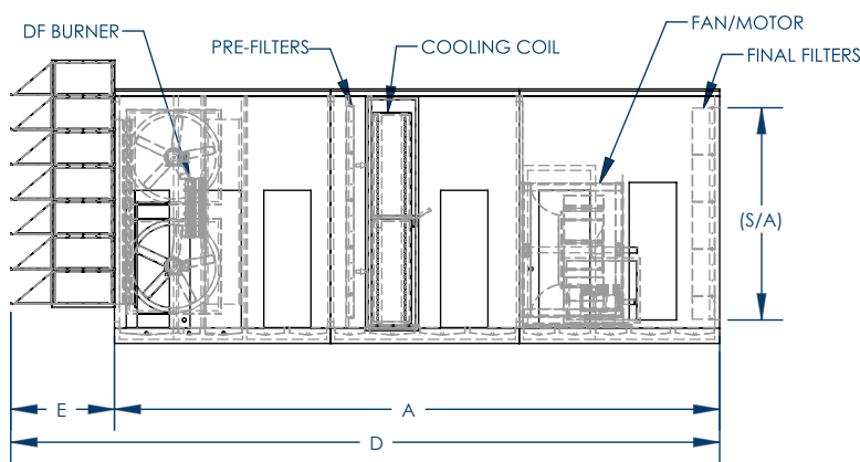
ELEVATION VIEW
